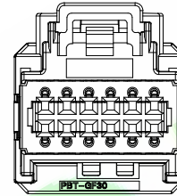
C Type Brown 12P
