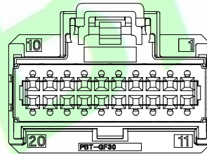
B Type Grey 20P
