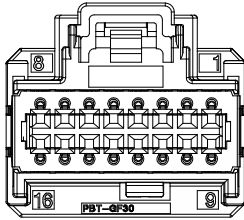
A Type Black 16P
