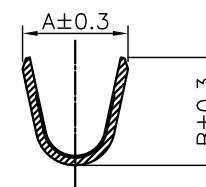
SECTION Z-Z
