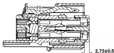
Primary Lock Reinforcement(PLR) Shown in Pre-Staged Position Section A-A
