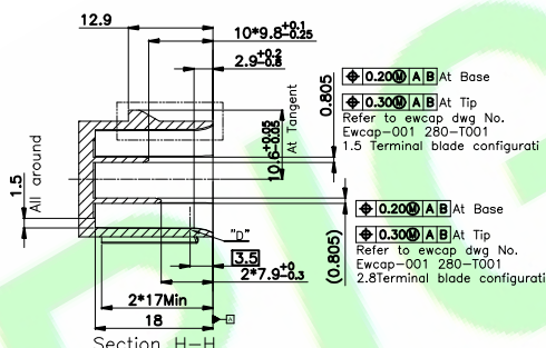
Section H-H
