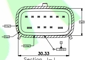
Section J-J
