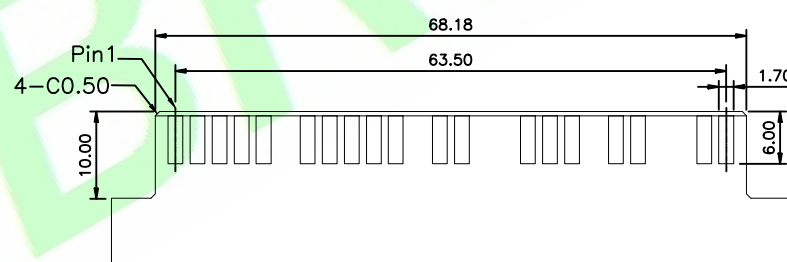
Recommended Plug-PCB layout (Tolerance:0.05mm)
