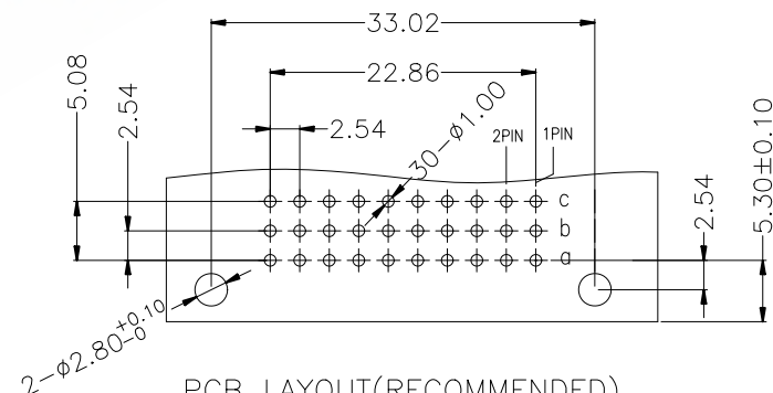
PCB LAYOUT(RECOMMENDED)
