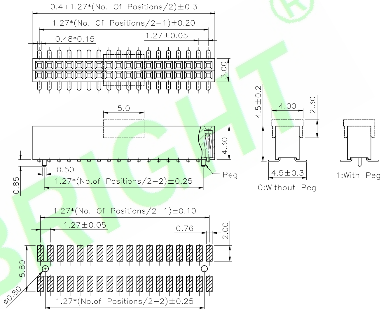
Recommended PCB Layout(Tolerance:0.05mm)
