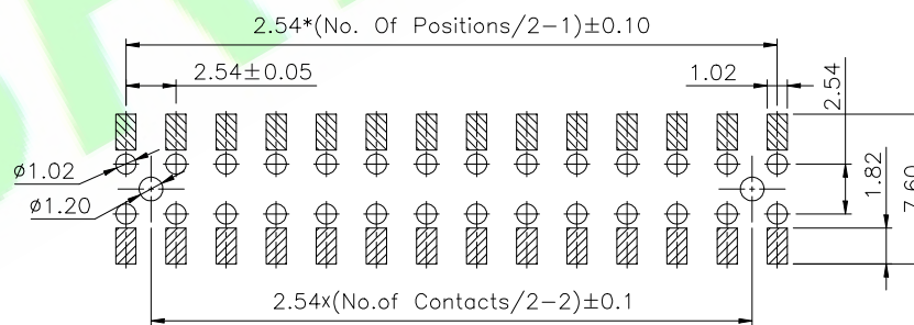
Recommended PCB Layout(Tolerance:0.05)
